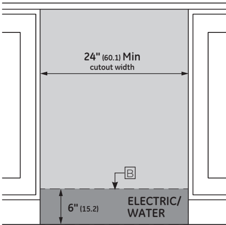
INSTALLATION CUTOUT FRONT VIEW
