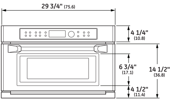
FRONT VIEW (SHOWING CUTOUT OVERLAP)
